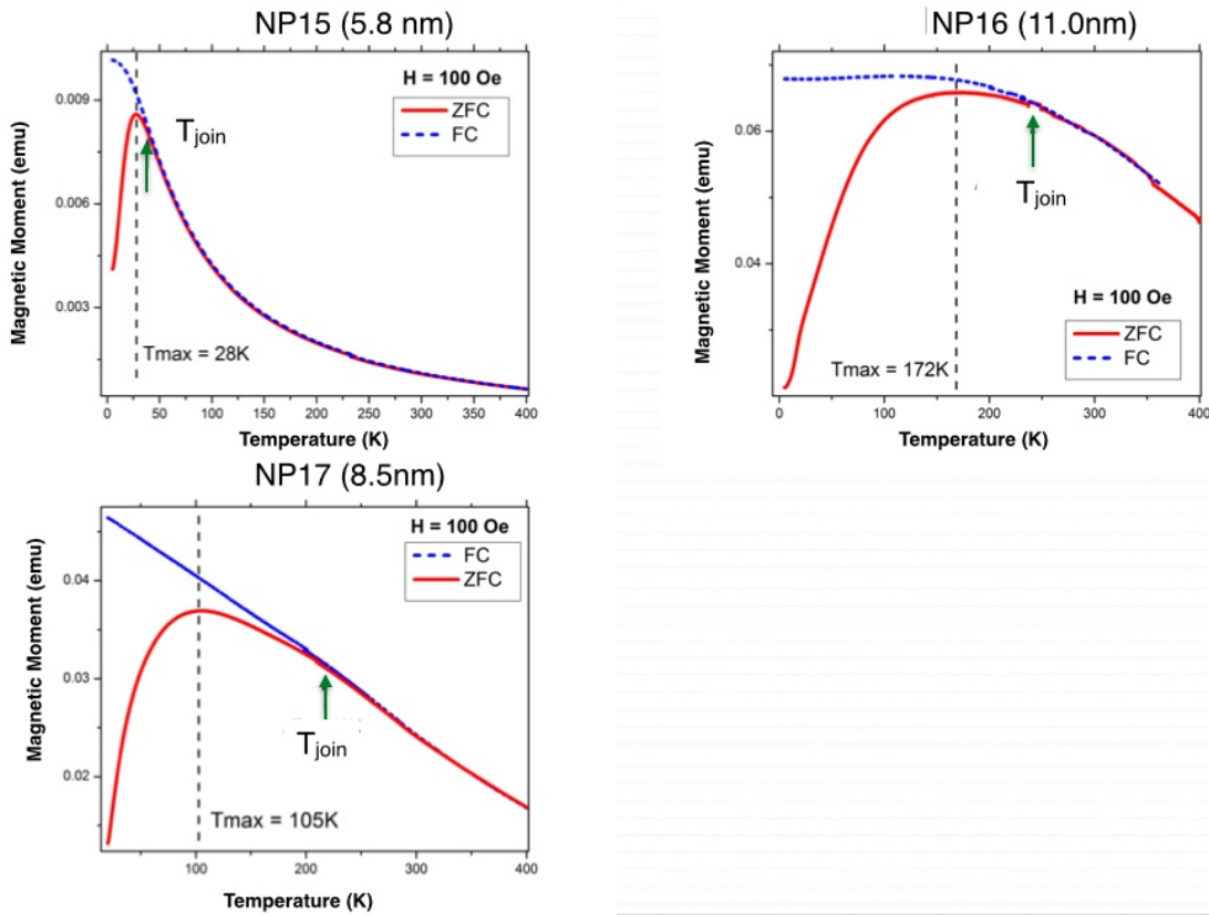
Figure 2.6 ZFC / FC measurements of sample NP15 (5nm), NP17 (8nm) and NP16 (11nm) measured at 100 Oe. T_{\text{max}} is the temperature when the magnetic moment of ZFC curve is at the maximum. T_{\text{join}} is the temperature when ZFC and FC curves join.
