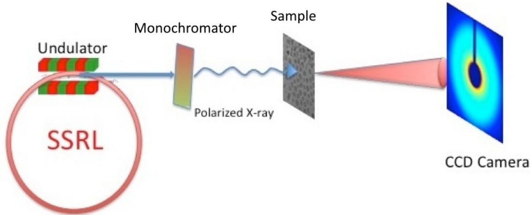
Figure 4.2 Sketch of the XRMS experiment. Coherent x-ray comes from SSRL is polarized by an undulator and tuned to the resonant edges of iron by a monochromator. X-ray is scattered by Fe_3O_4 assemble and detected by a CCD camera.
